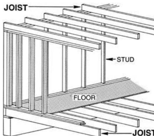
Rajah 2.4.15 Joist
