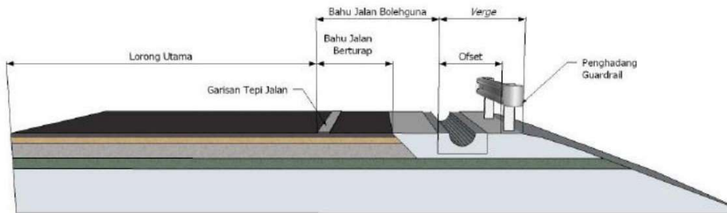
Figure 9. Paved road shoulder structure
