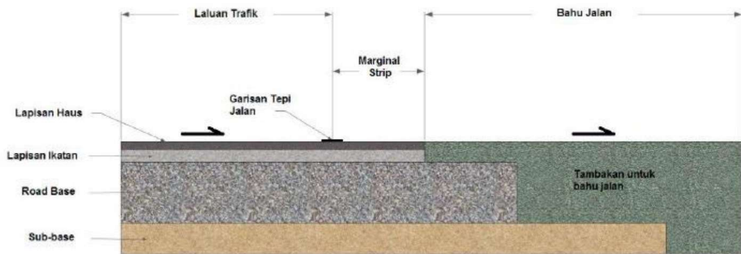
Figure 10. Unpaved road shoulder structure.
